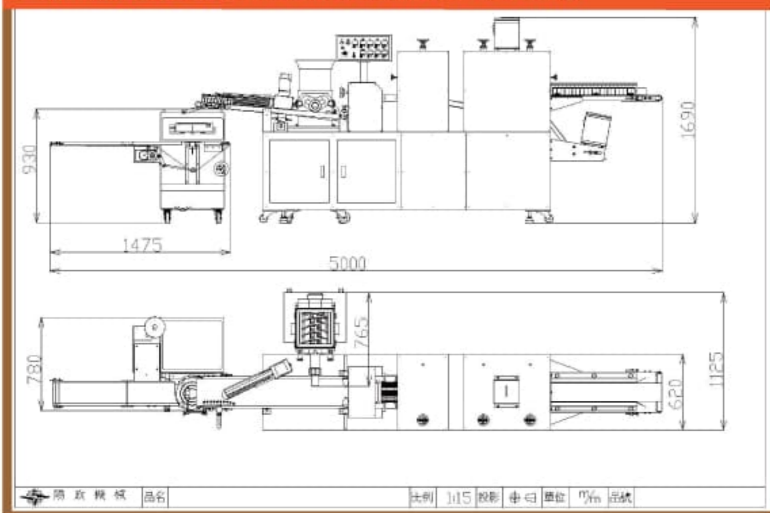
产品规格尺寸图 Specification and Dimension Drawing
